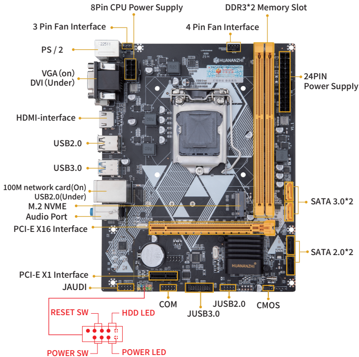
1-1 H81 Motherboard Illustration
